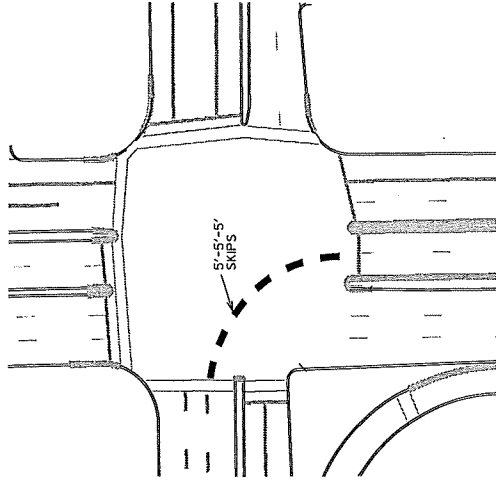
TURN RADIUS LINE DETAILS
