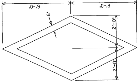
RESTRICTED LANE SYMBOL
